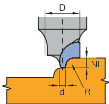
Inner contour with radii
