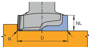
Face milling with rounded corners
