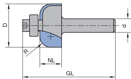
Guttering mould cutter with guide ring
