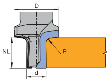
Outer contour with radii
