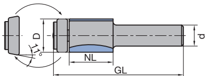
Edge trimming cutter with guide ring on bottom
